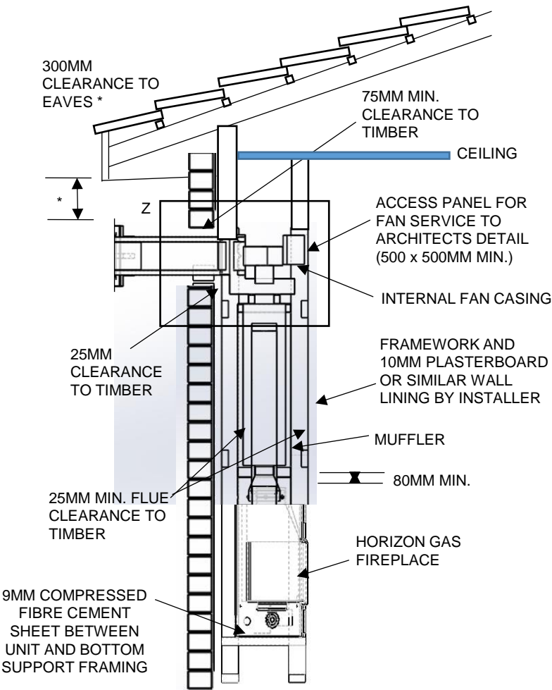
DETAIL Z
