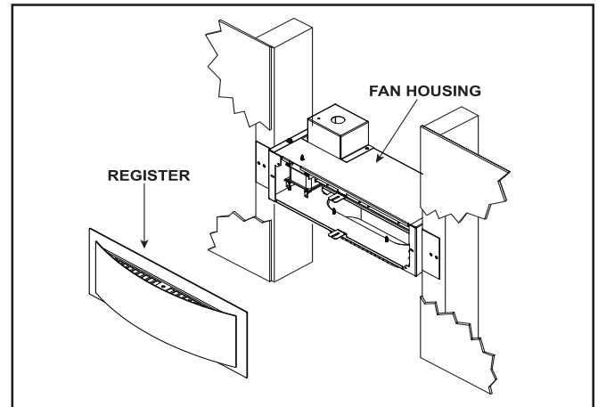
Figure 5.11 Register Attachment
