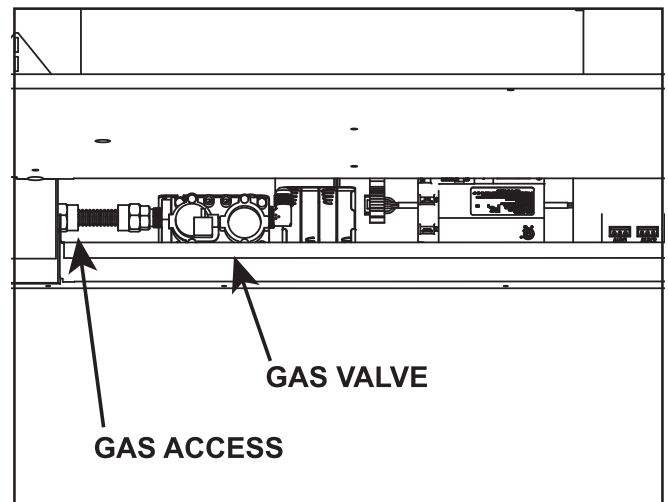
Figure 9.5. Gas Fitting Access with Vanity Panel Removed
