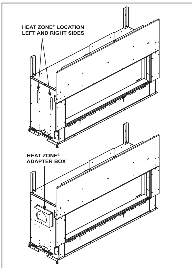
Figure 5.6 Adapter Box
