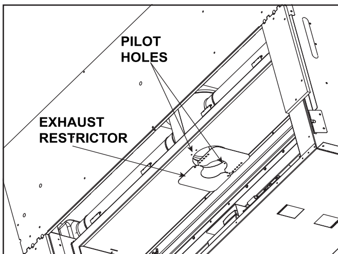
Figure 4.5 Exhaust Restrictor
