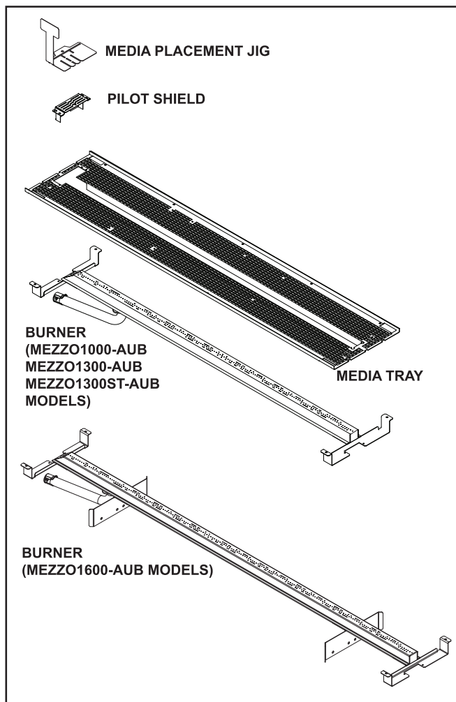
→ Figure 9.3. Media Tray with Burner and Pilot Shield
