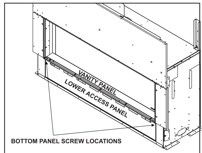
Figure 9.2. Vanity Panel and Lower Access Panel Location
