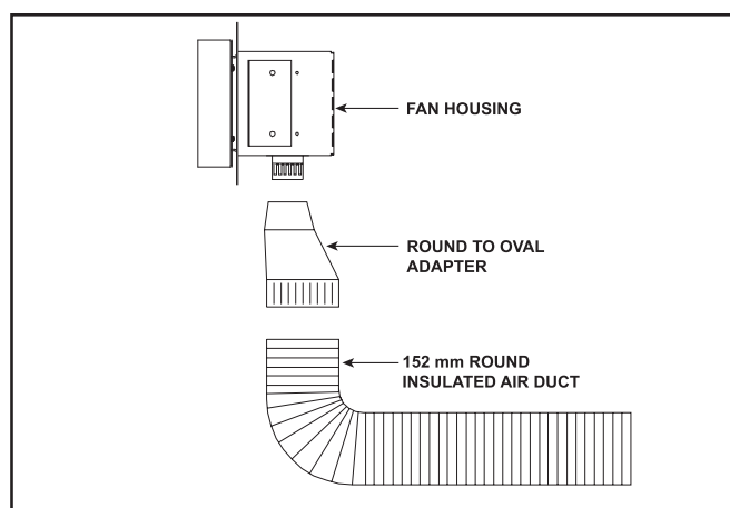
Figure 5.9 Duct Attachment
