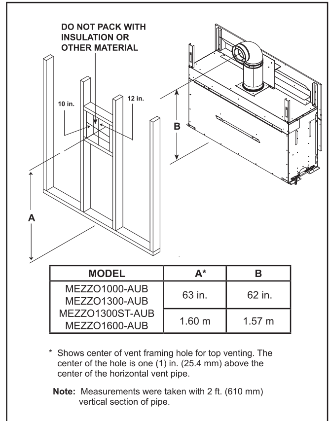
Figure 5.2 Wall Penetration
