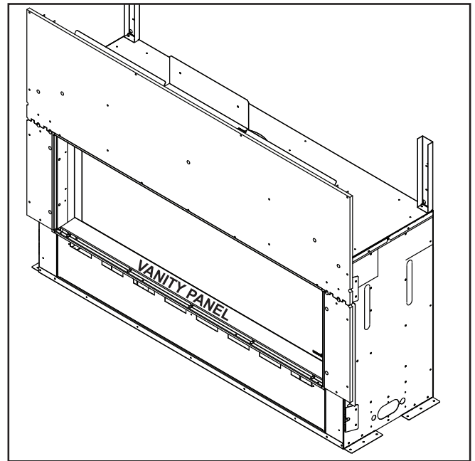
Figure 11.2 Vanity Panel Location
