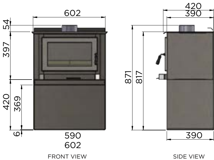
STACK
