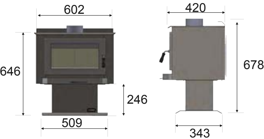
PEDESTAL
